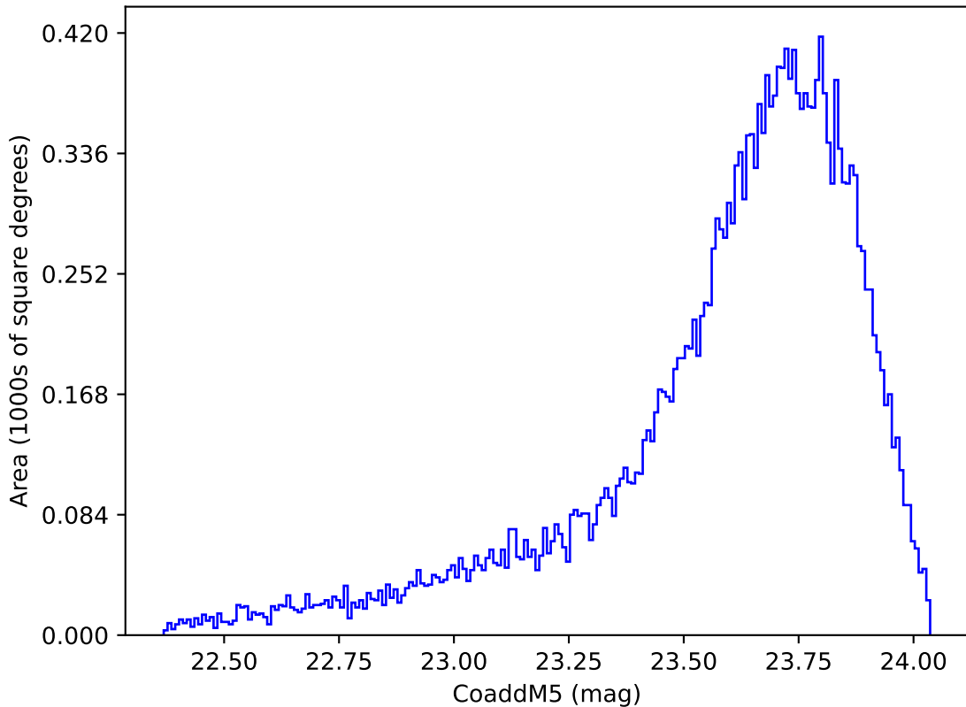
early_u_fpextra3.0_v3.4_10yrs Yr 1 y band: CoaddM5
