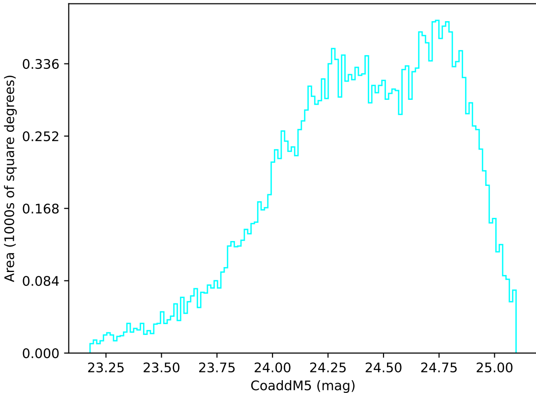
early_u_fpextra3.0_v3.4_10yrs Yr 1 u band: CoaddM5
