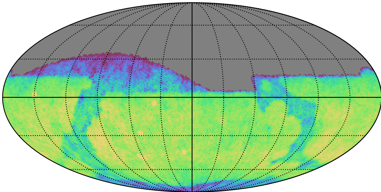
early_u_fpextra3.0_v3.4_10yrs Yr 1 r band: CoaddM5
