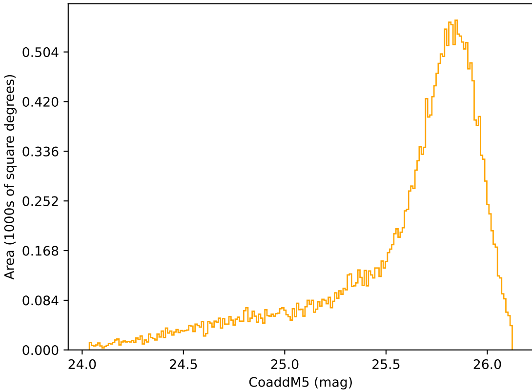
early_u_fpextra3.0_v3.4_10yrs Yr 1 r band: CoaddM5
