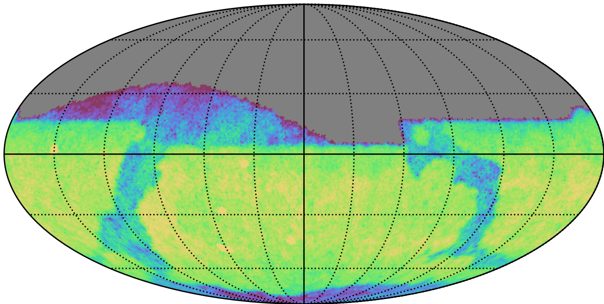
early_u_fpextra3.0_v3.4_10yrs Yr 1 i band: CoaddM5
