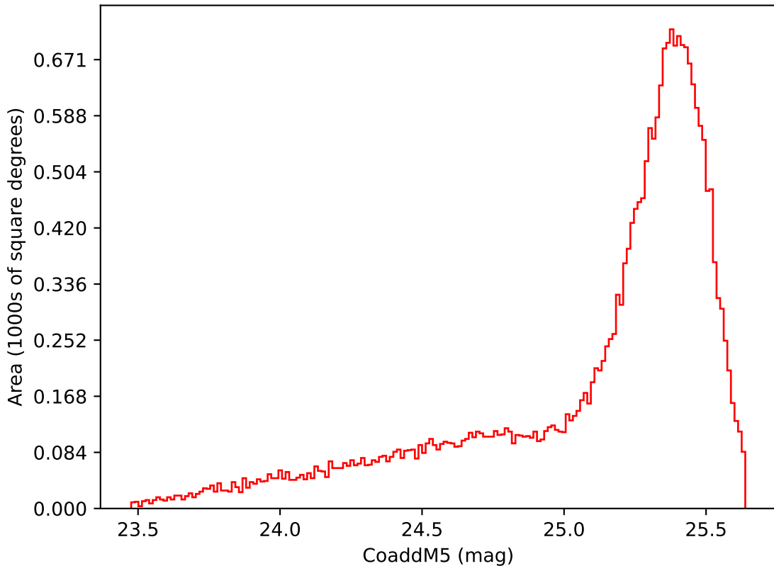
early_u_fpextra3.0_v3.4_10yrs Yr 1 i band: CoaddM5
