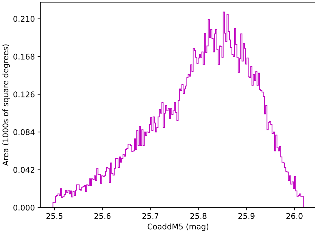
early_u_fpextra3.0_v3.4_10yrs WFD z band: CoaddM5
