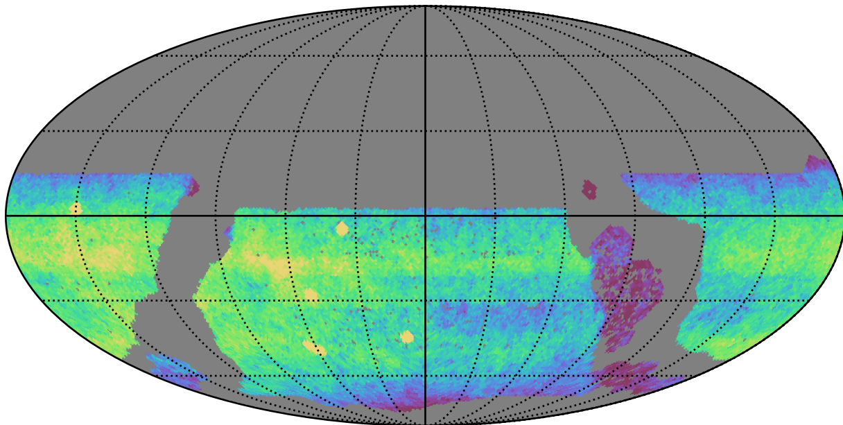
early_u_fpextra3.0_v3.4_10yrs WFD u band: CoaddM5
