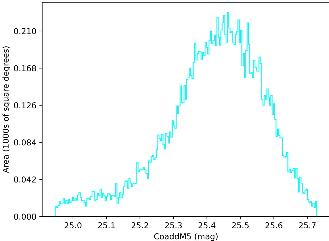
early_u_fpextra3.0_v3.4_10yrs WFD u band: CoaddM5
