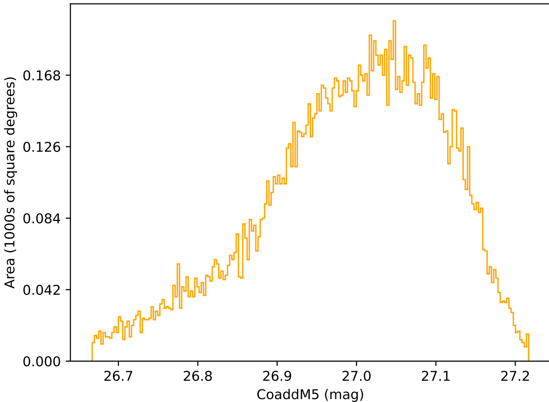
early_u_fpextra3.0_v3.4_10yrs WFD r band: CoaddM5
