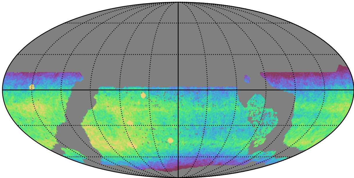
early_u_fpextra3.0_v3.4_10yrs WFD i band: CoaddM5
