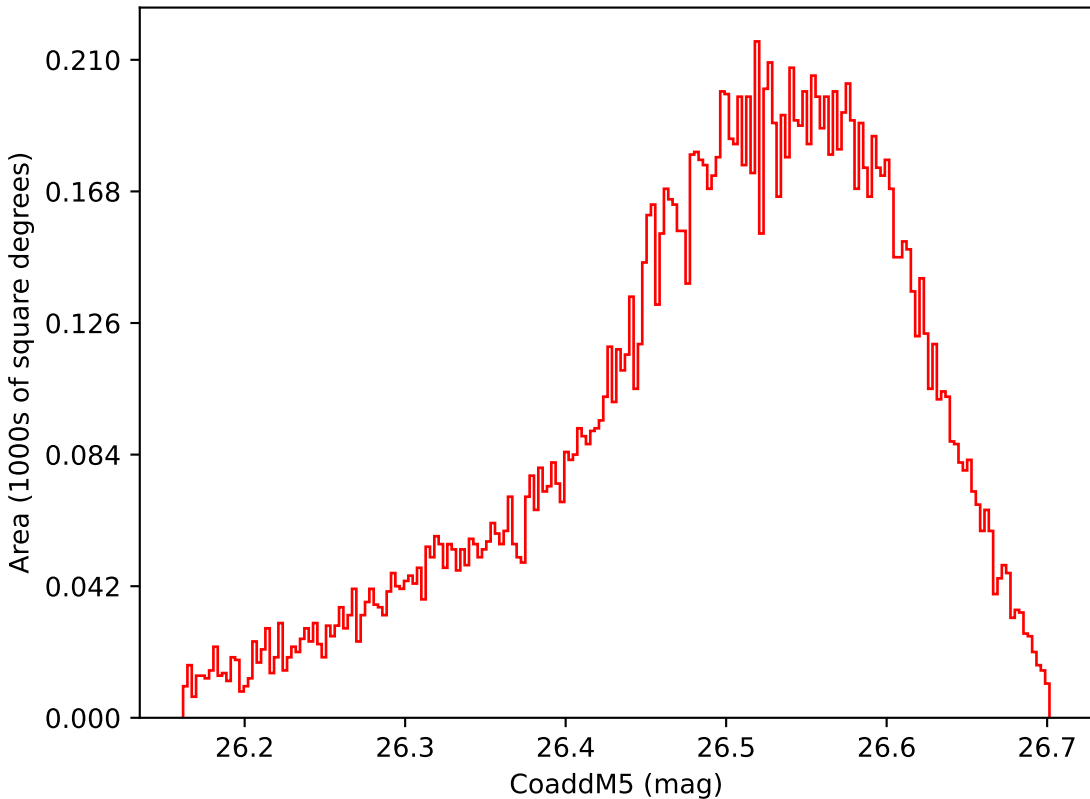
early_u_fpextra3.0_v3.4_10yrs WFD i band: CoaddM5
