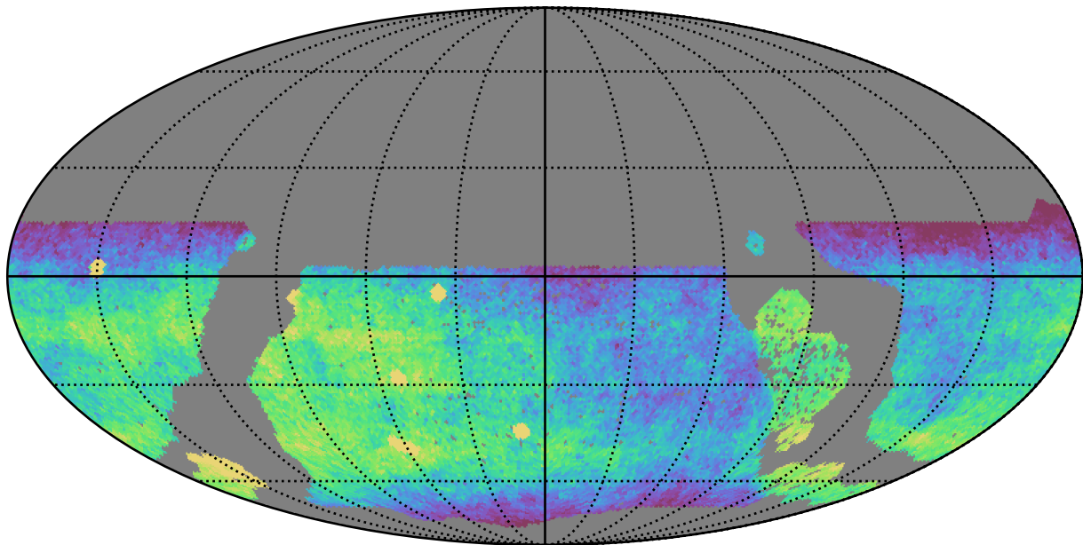
early_u_fpextra3.0_v3.4_10yrs WFD g band: CoaddM5
