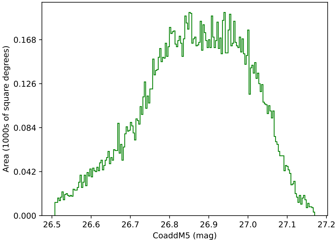
early_u_fpextra3.0_v3.4_10yrs WFD g band: CoaddM5
