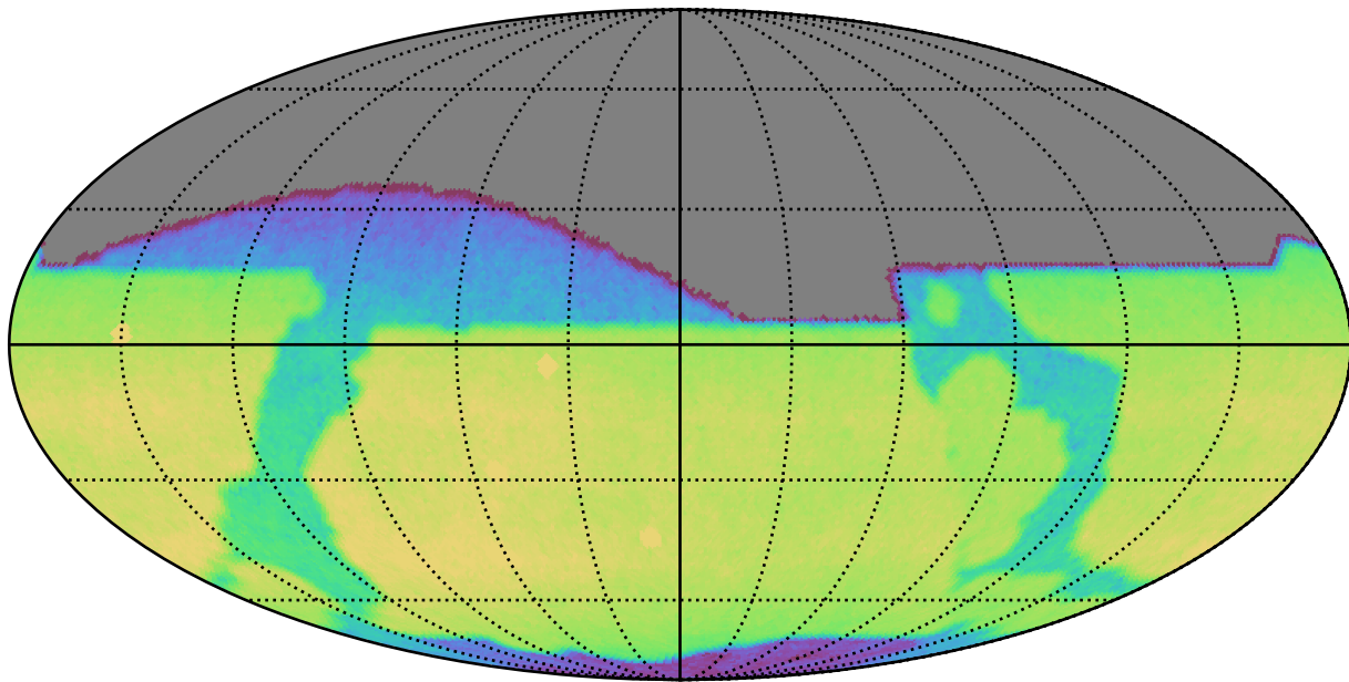
early_u_fpextra3.0_v3.4_10yrs All sky z band: CoaddM5
