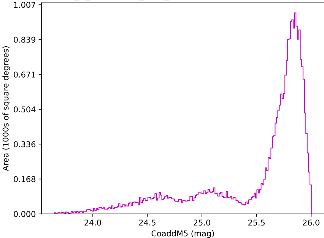
early_u_fpextra3.0_v3.4_10yrs All sky z band: CoaddM5
