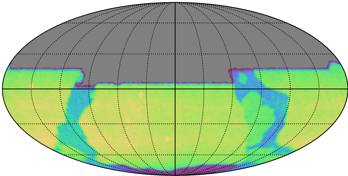
early_u_fpextra3.0_v3.4_10yrs All sky y band: CoaddM5
