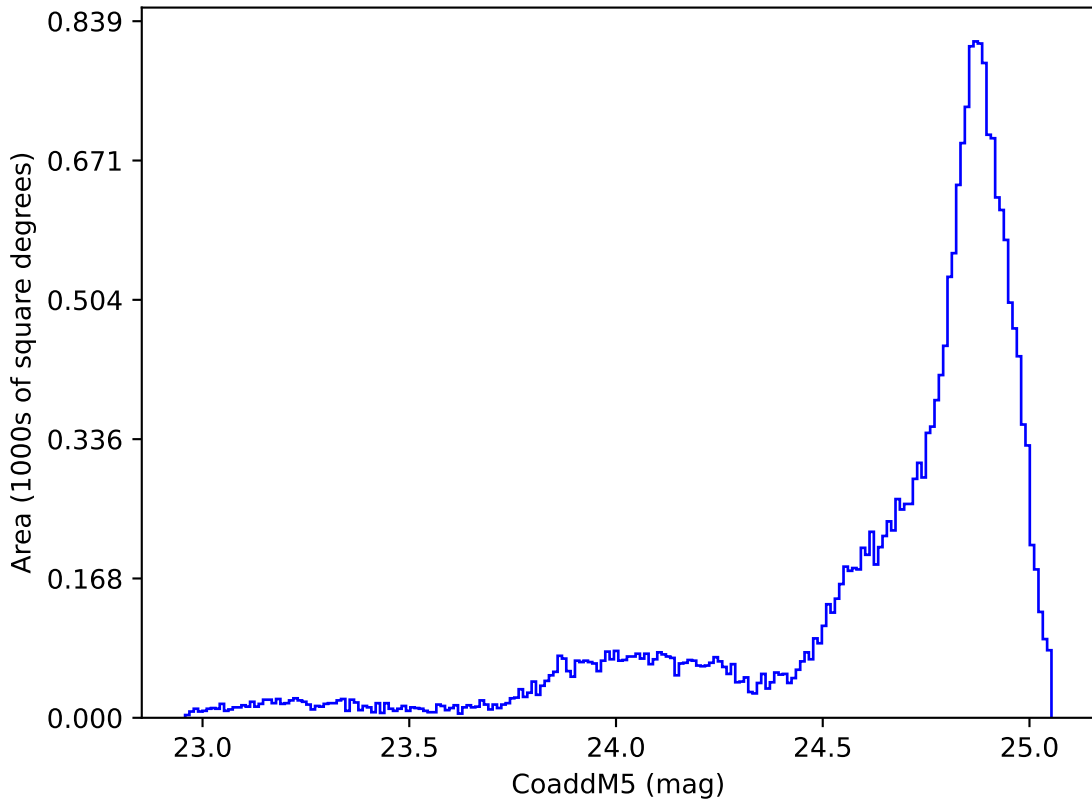
early_u_fpextra3.0_v3.4_10yrs All sky y band: CoaddM5
