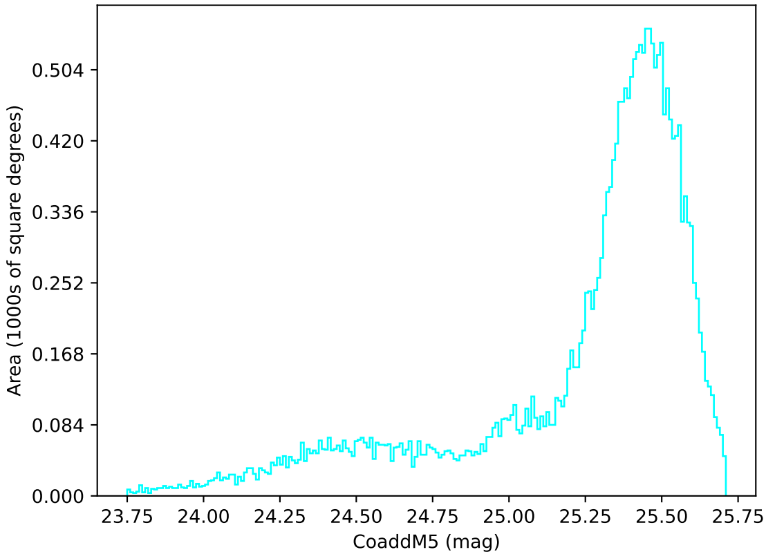
early_u_fpextra3.0_v3.4_10yrs All sky u band: CoaddM5
