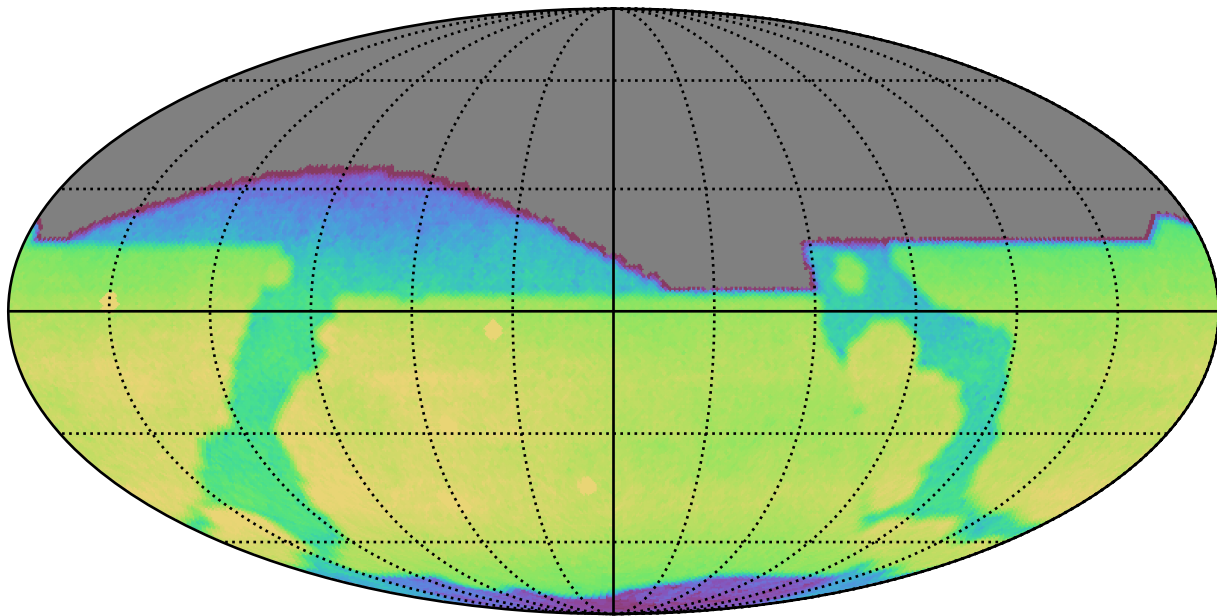
early_u_fpextra3.0_v3.4_10yrs All sky r band: CoaddM5
