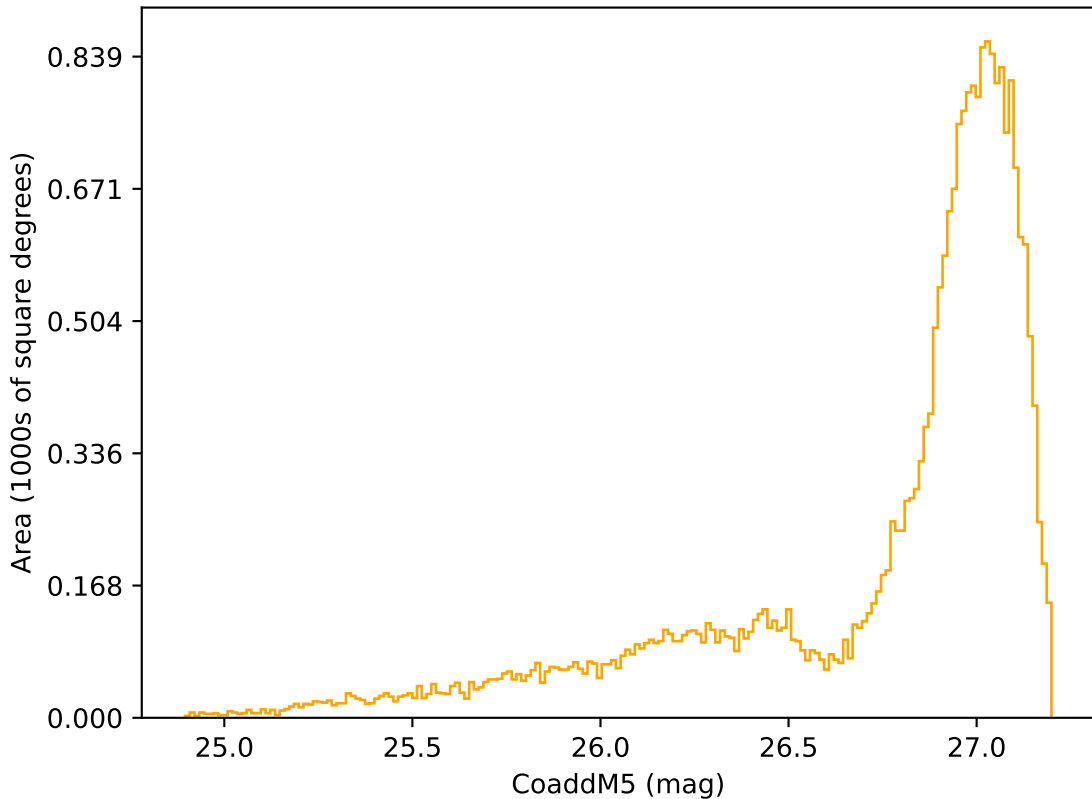
early_u_fpextra3.0_v3.4_10yrs All sky r band: CoaddM5
