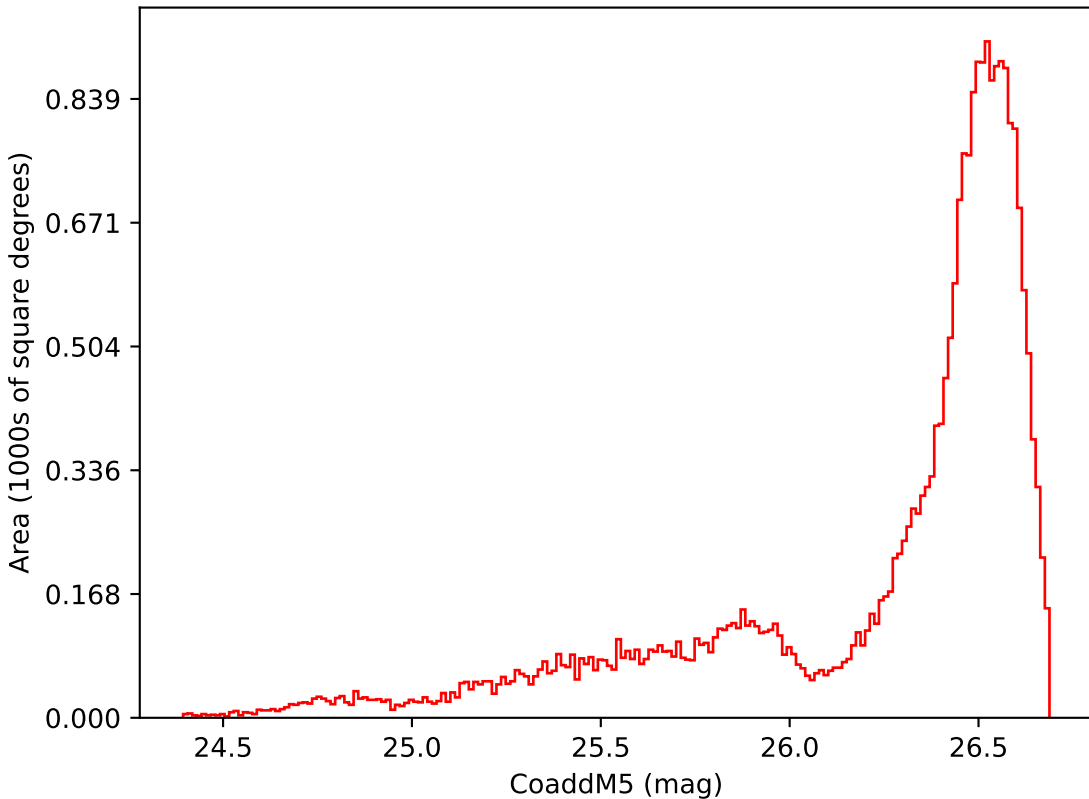
early_u_fpextra3.0_v3.4_10yrs All sky i band: CoaddM5
