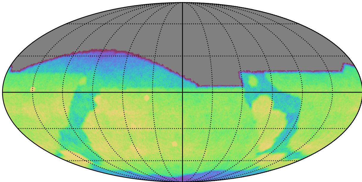
early_u_fpextra3.0_v3.4_10yrs All sky g band: CoaddM5
