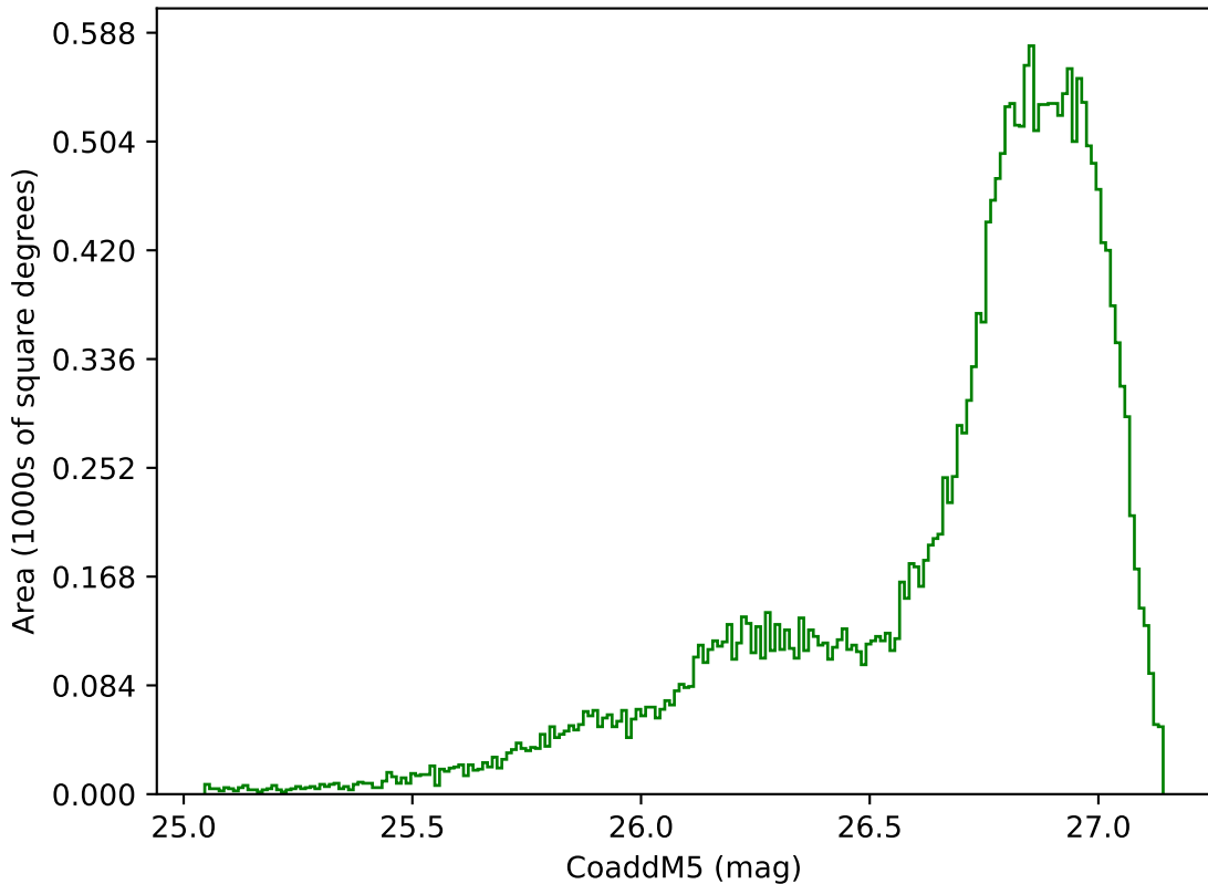
early_u_fpextra3.0_v3.4_10yrs All sky g band: CoaddM5
