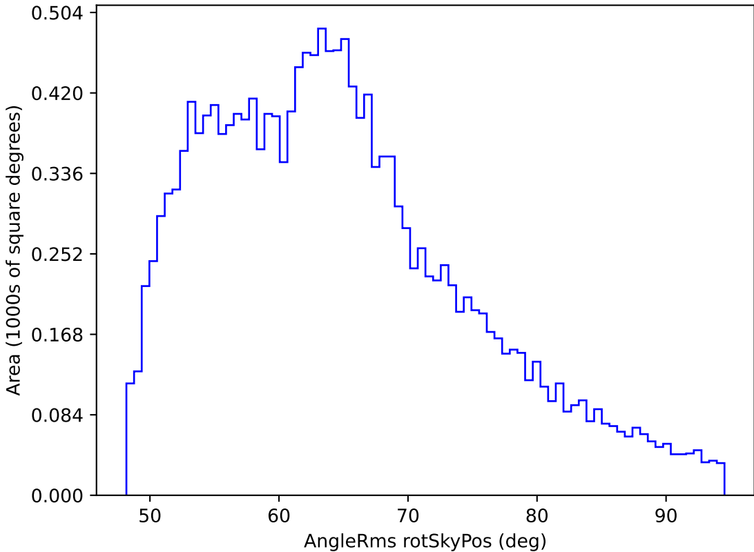
early_u_fpextra3.0_v3.4_10yrs WFD z band: AngleRms rotSkyPos
