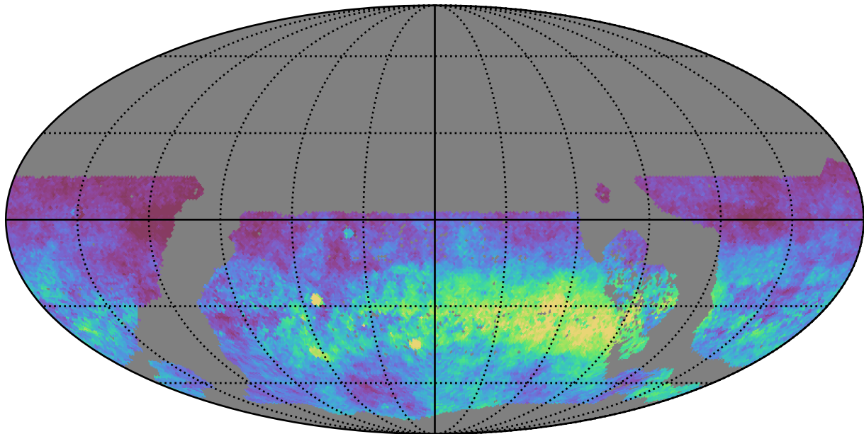
early_u_fpextra3.0_v3.4_10yrs WFD y band: AngleRms rotSkyPos
