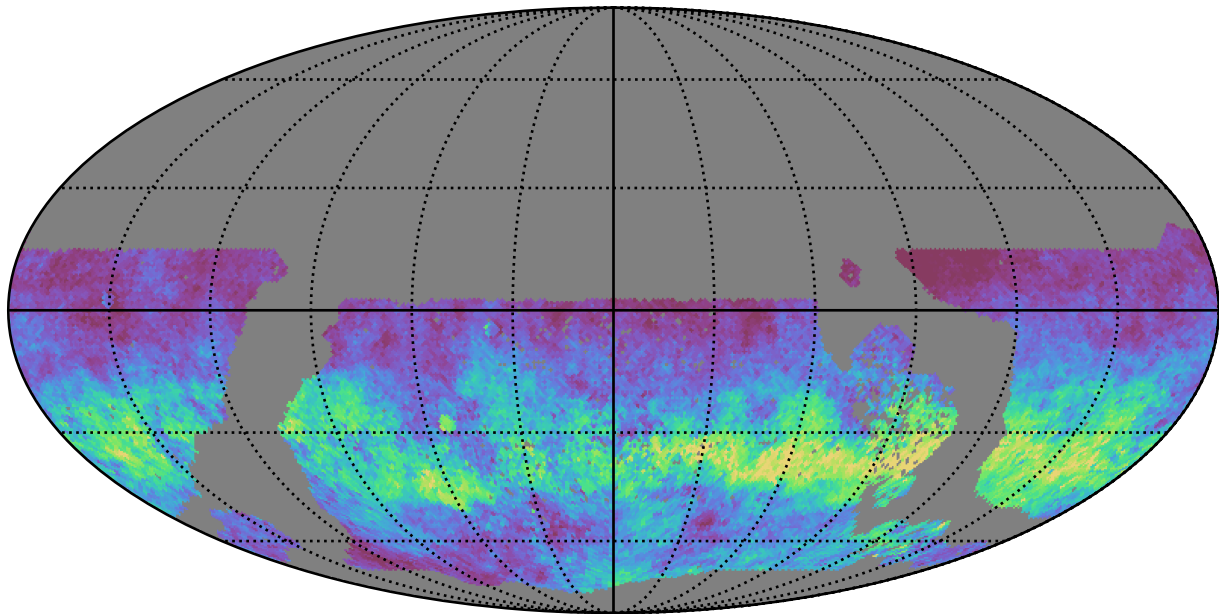
early_u_fpextra3.0_v3.4_10yrs WFD u band: AngleRms rotSkyPos
