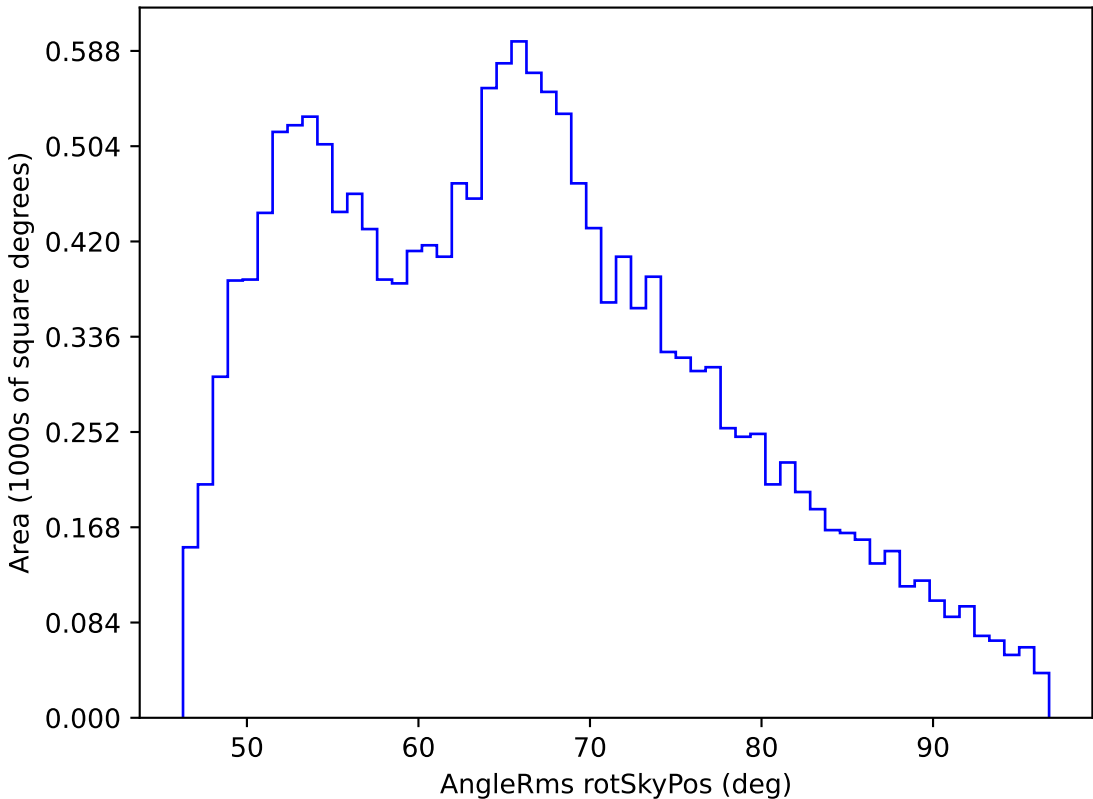
early_u_fpextra3.0_v3.4_10yrs WFD r band: AngleRms rotSkyPos
