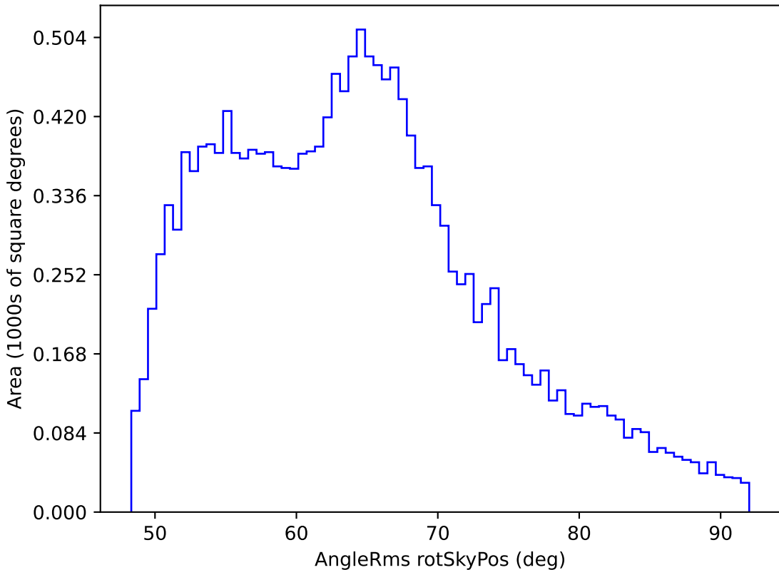
early_u_fpextra3.0_v3.4_10yrs WFD i band: AngleRms rotSkyPos
