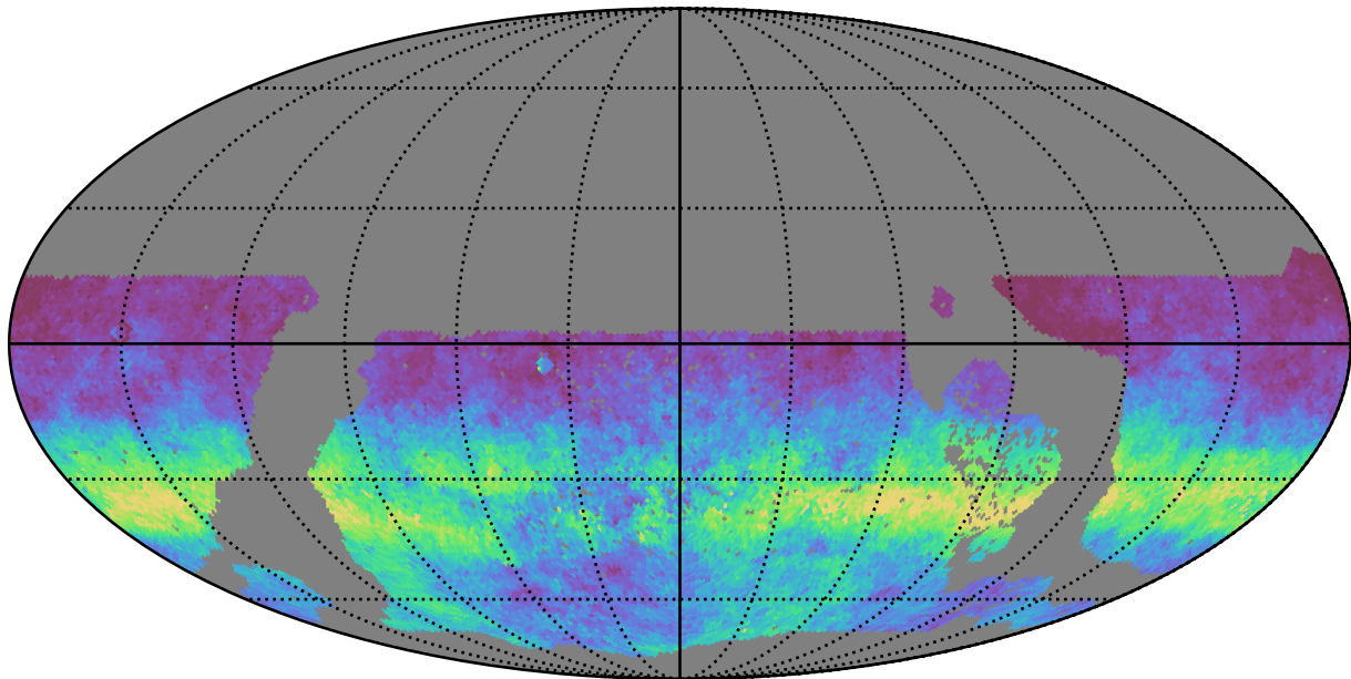
early_u_fpextra3.0_v3.4_10yrs WFD g band: AngleRms rotSkyPos
