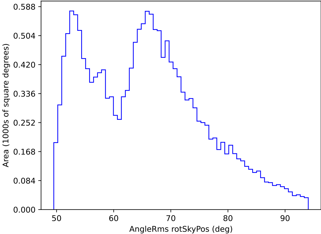
early_u_fpextra3.0_v3.4_10yrs WFD all bands: AngleRms rotSkyPos
