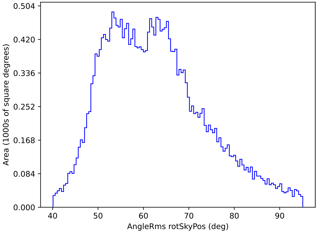
early_u_fpextra3.0_v3.4_10yrs All sky z band: AngleRms rotSkyPos
