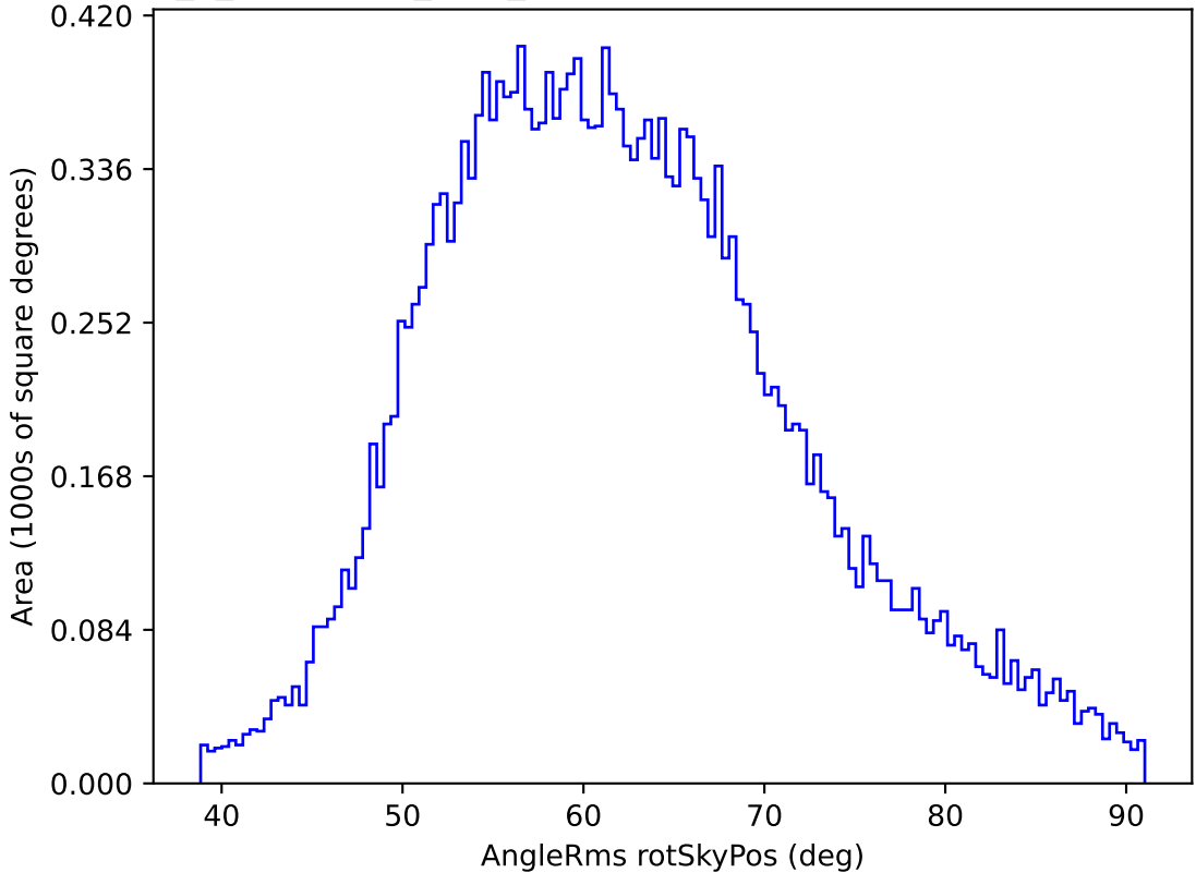
early_u_fpextra3.0_v3.4_10yrs All sky y band: AngleRms rotSkyPos
