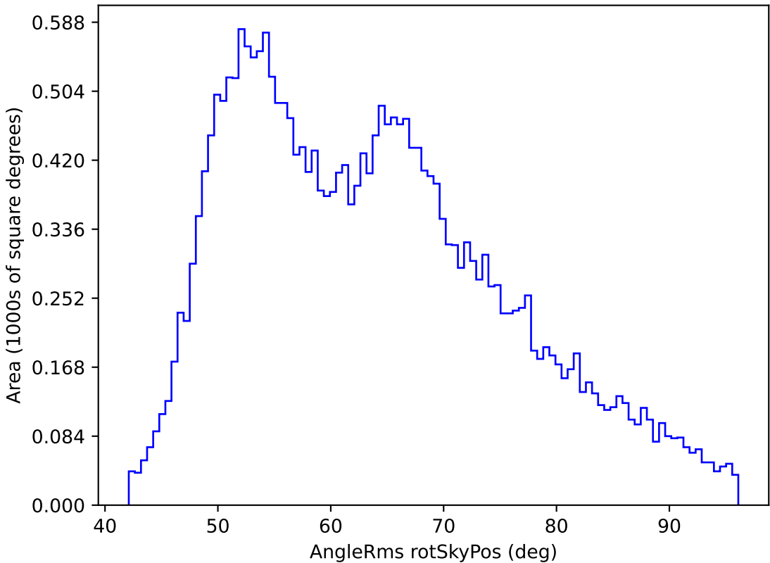
early_u_fpextra3.0_v3.4_10yrs All sky r band: AngleRms rotSkyPos
