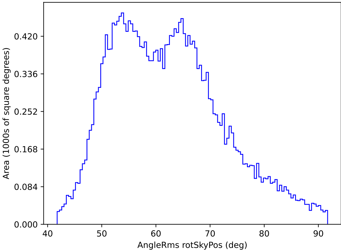
early_u_fpextra3.0_v3.4_10yrs All sky i band: AngleRms rotSkyPos
