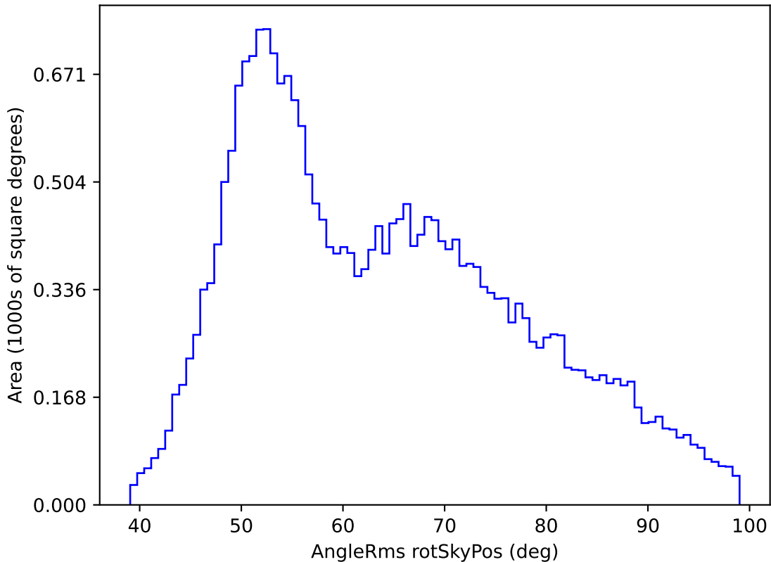
early_u_fpextra3.0_v3.4_10yrs All sky g band: AngleRms rotSkyPos
