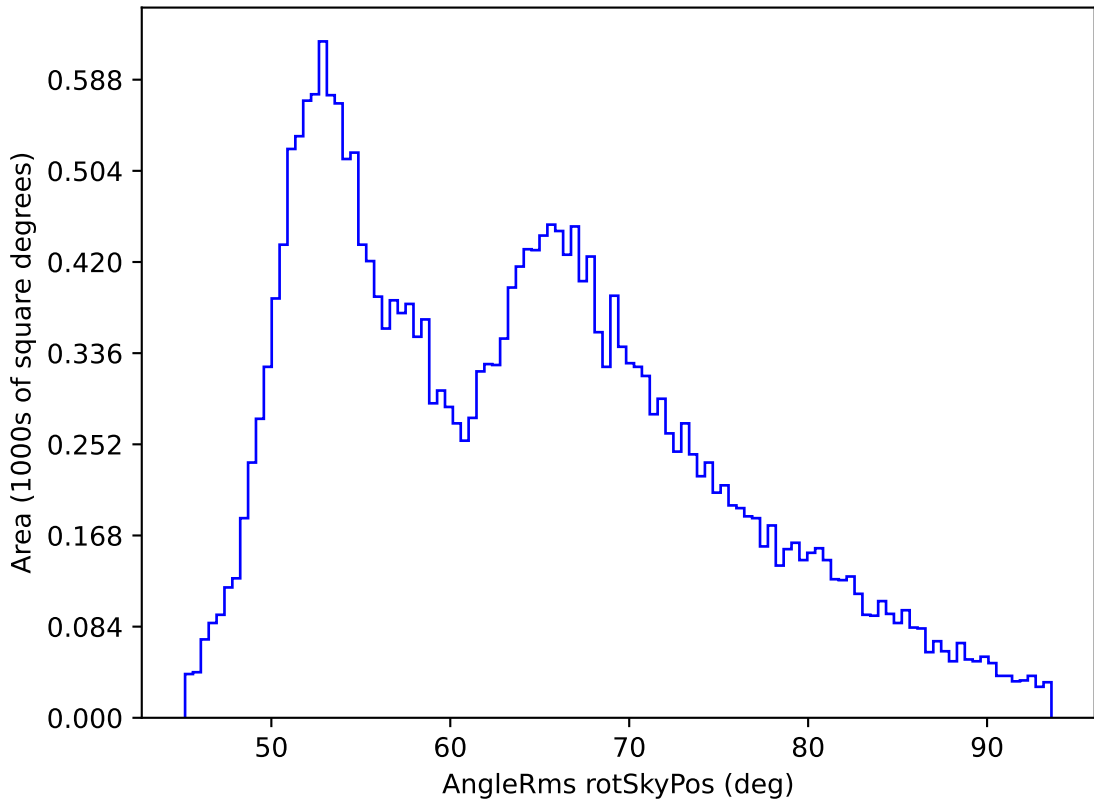
early_u_fpextra3.0_v3.4_10yrs All sky all bands: AngleRms rotSkyPos
