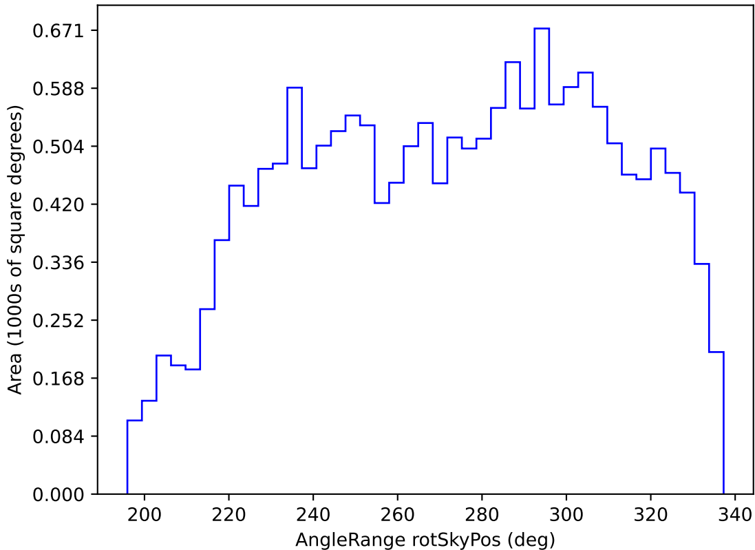
early_u_fpextra3.0_v3.4_10yrs WFD y band: AngleRange rotSkyPos
