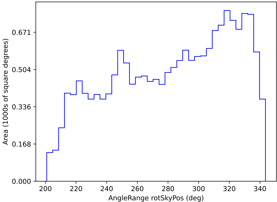
early_u_fpextra3.0_v3.4_10yrs WFD r band: AngleRange rotSkyPos
