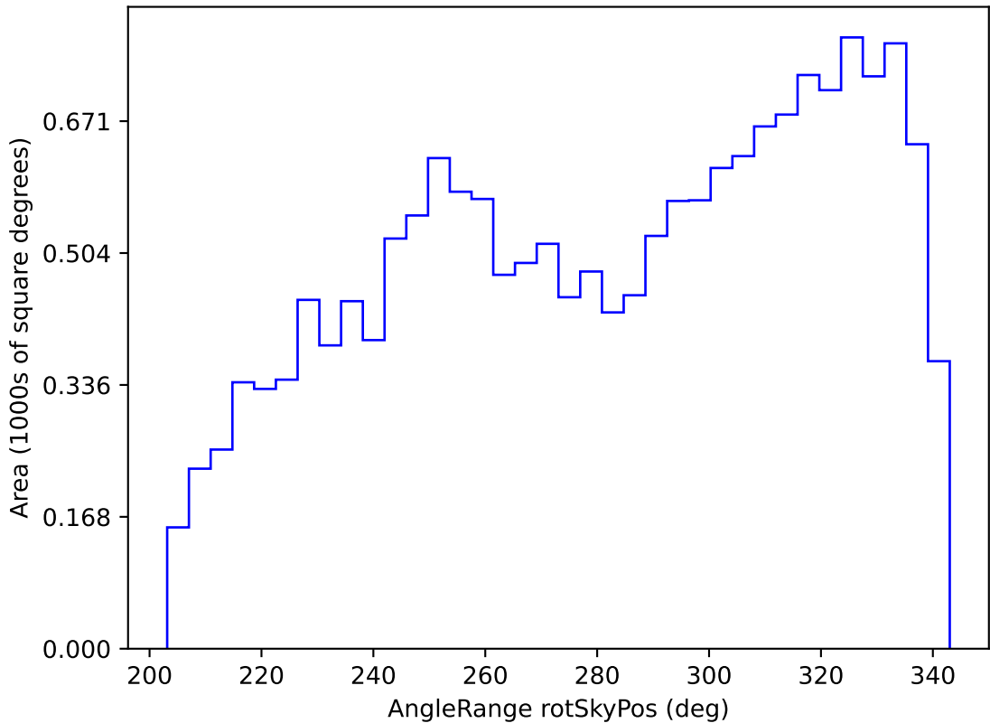
early_u_fpextra3.0_v3.4_10yrs WFD i band: AngleRange rotSkyPos
