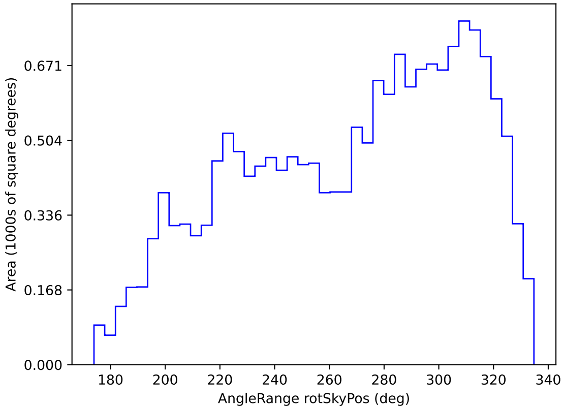
early_u_fpextra3.0_v3.4_10yrs WFD g band: AngleRange rotSkyPos
