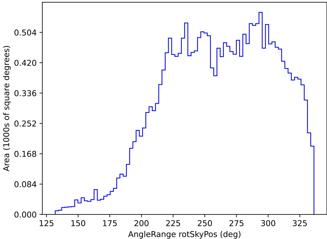
early_u_fpextra3.0_v3.4_10yrs All sky y band: AngleRange rotSkyPos
