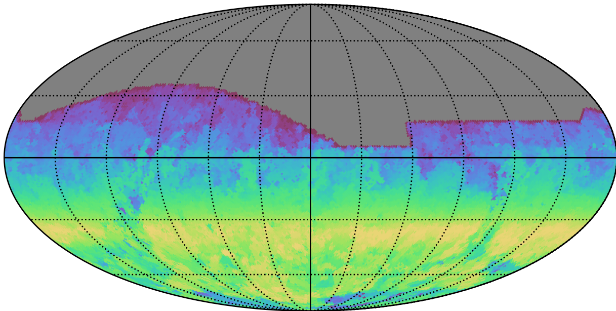
early_u_fpextra3.0_v3.4_10yrs All sky r band: AngleRange rotSkyPos
