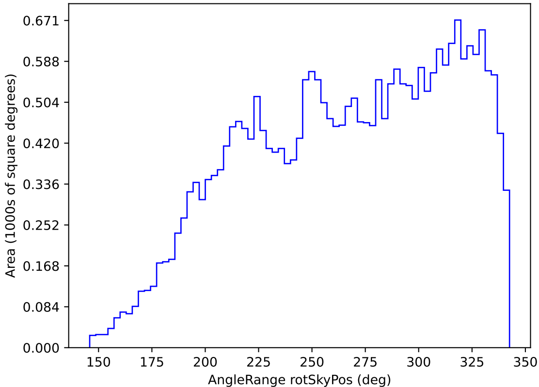
early_u_fpextra3.0_v3.4_10yrs All sky r band: AngleRange rotSkyPos
