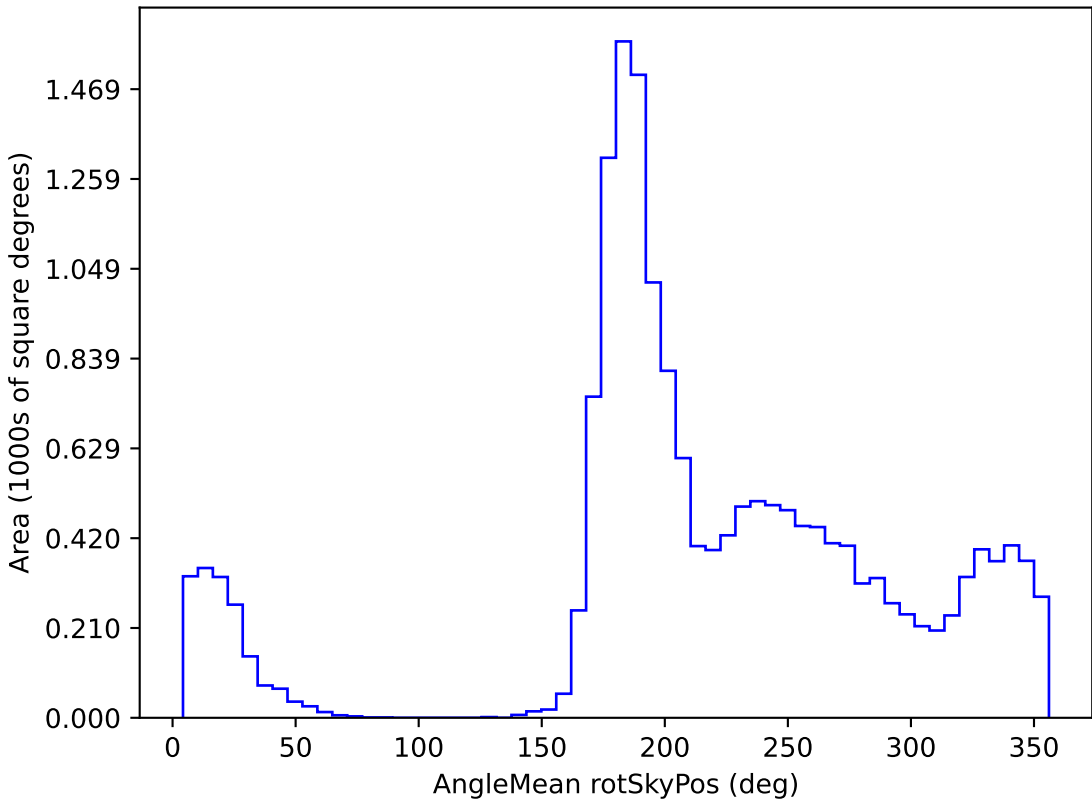
early_u_fpextra3.0_v3.4_10yrs WFD u band: AngleMean rotSkyPos
