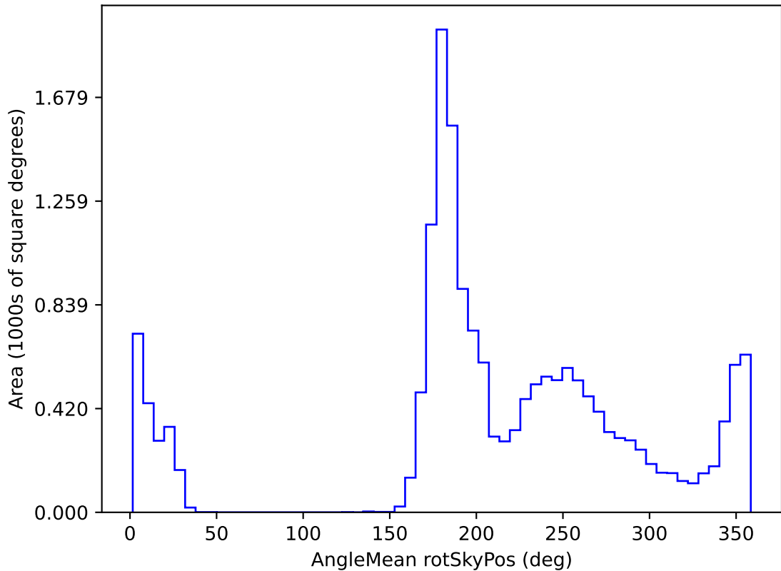
early_u_fpextra3.0_v3.4_10yrs WFD i band: AngleMean rotSkyPos
