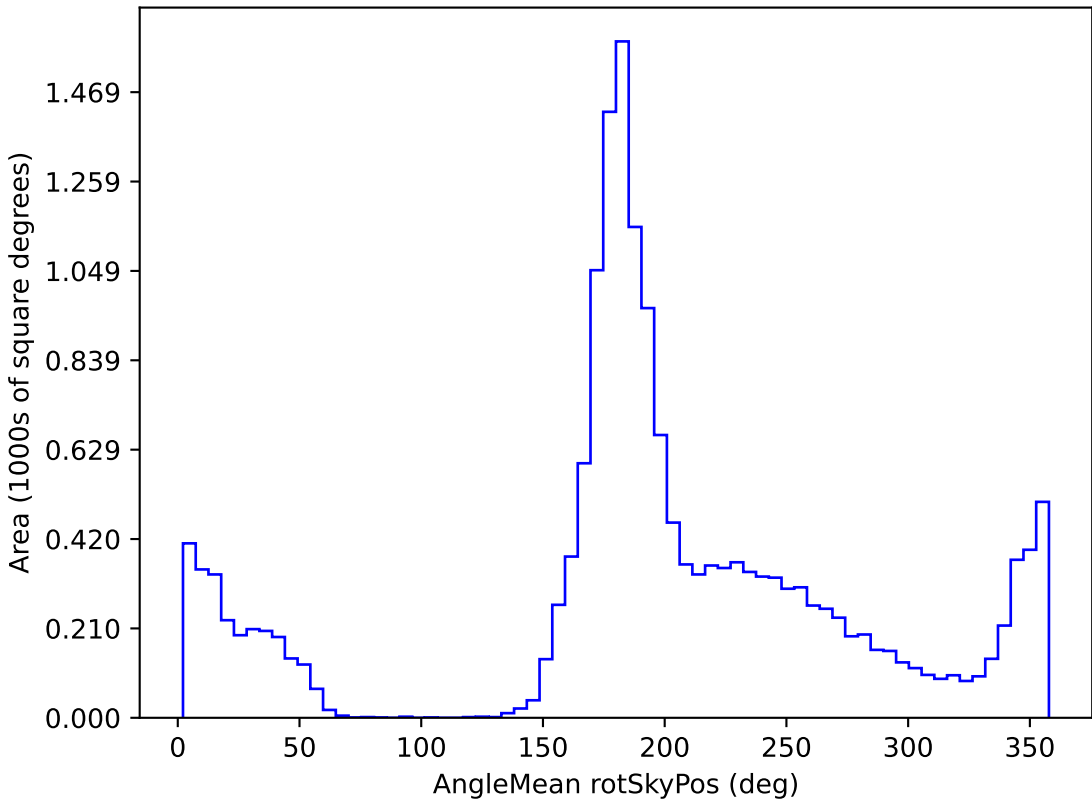
early_u_fpextra3.0_v3.4_10yrs WFD g band: AngleMean rotSkyPos
