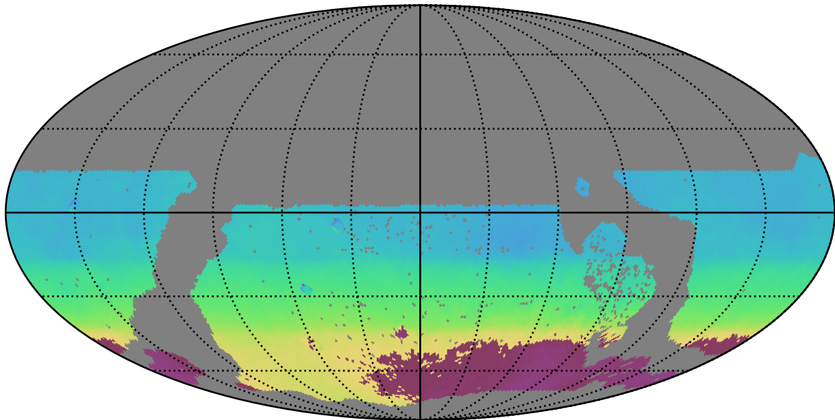
early_u_fpextra3.0_v3.4_10yrs WFD all bands: AngleMean rotSkyPos
