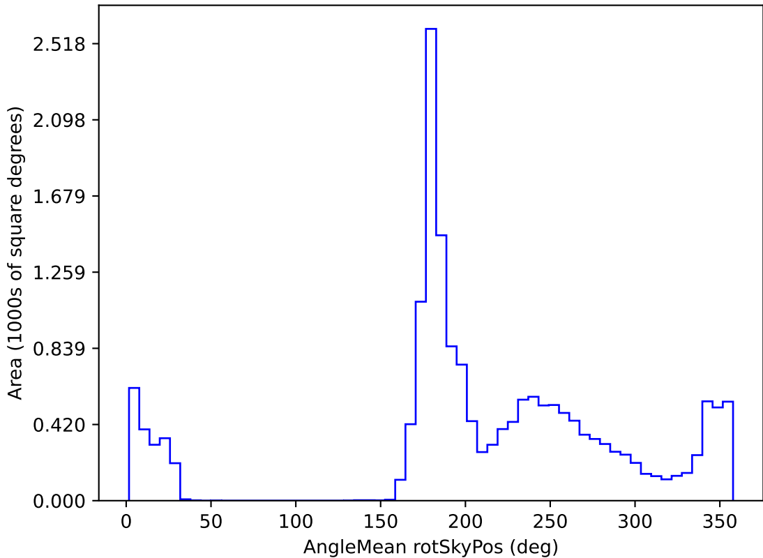
early_u_fpextra3.0_v3.4_10yrs WFD all bands: AngleMean rotSkyPos
