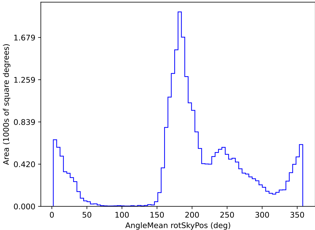
early_u_fpextra3.0_v3.4_10yrs All sky z band: AngleMean rotSkyPos
